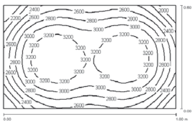
1 x SLE 2x36W TC-L + 2 x SLKE 1x36W TC-L E_{max} = 3426 \text{ lx}
