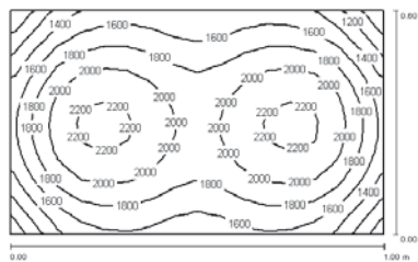
2 x SLKE 1x36W TC-L E_{max} = 2276 \text{ lx}
